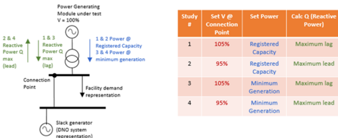
Figure 13: Example of Type C and D PGM Reactive Capability Studies.
